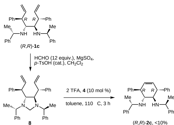
Scheme 3. RCM reaction of the diaminodiene ( R,R )- 1c .
