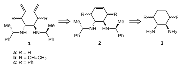
Scheme 1. Synthetic route to 3,6-disubstituted 1,2-diamino-cyclohexanes.
