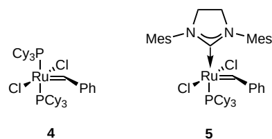
Figure 1. Ruthenium carbene complexes used for RCM reactions.
