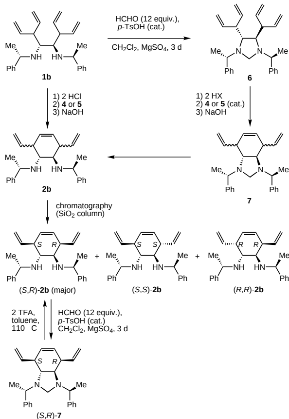
Scheme 2. Diastereoselective RCM reactions of diaminotetraene derivatives.
